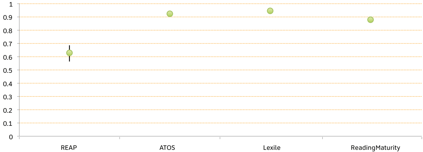
Figure 5.1.5-1: Oasis passages, Correlation with empirical Lexile (n=372)
